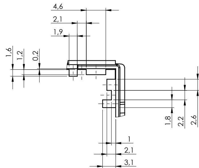
DETAIL D SCALE 2 : 1
