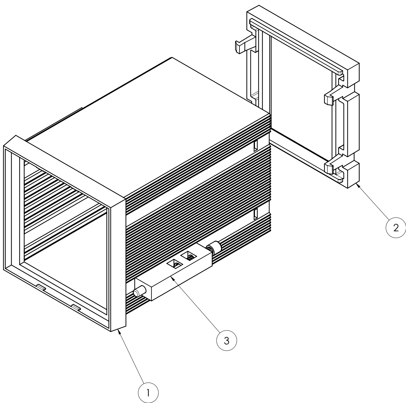
GENERAL ASSEMBLY EXPLODED VIEW
