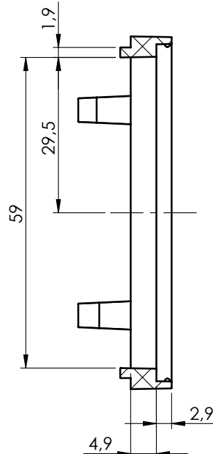
SECTION B-B
