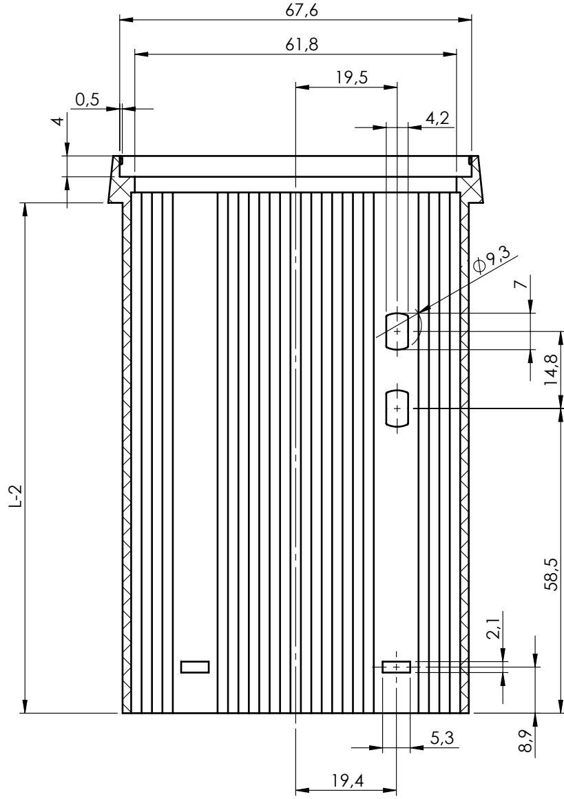
SECTION C-C
